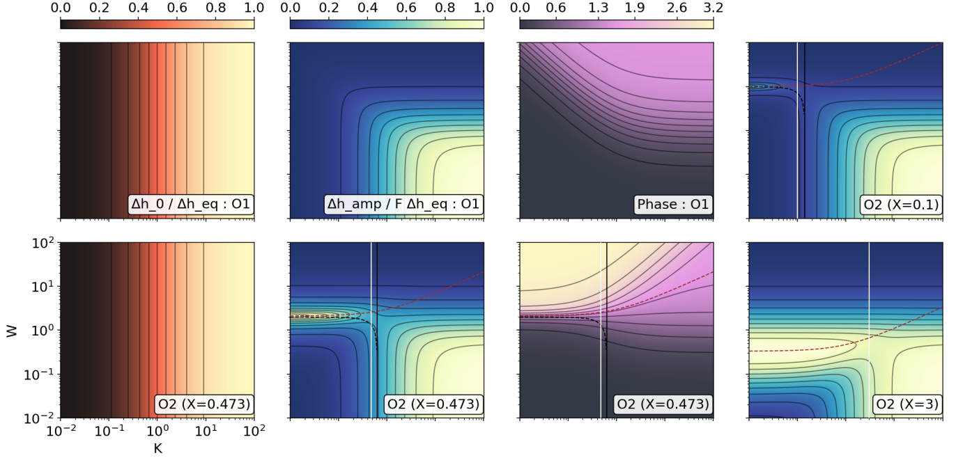
Figure 4. First and second order response of tidally-locked planets to variable heating, showing forcing normalized time-mean height magnitude ( \Delta h_o/\Delta h_{eq} ), its amplitude ( \Delta h_{amp}/F\Delta h_o ), and phase lag of the response using different colorschemes. The first order (O1) is dependent only on two nondimensional parameters W = \omega\tau_{rad} and K , while the second order (O2) has a third parameter X = \tau_{wave}/\tau_{rad} . The magnitude responses for both are the same and commensurate with D. Perez-Becker & A. P. Showman (2013) . The brown and black dashed lines correspond to natural ( \Omega_o ) and resonant ( \Omega_{res} ) frequencies of the system. The solid black line corresponds to the critical damping K , to the left of which oscillatory solutions exist, and the system is overdamped to the right. The solid white line represents separation between the wave dominated inertial regime to the left of it and the drag/rotation dominated regime to the right, where the solutions match the first-order theory.
