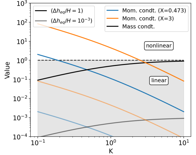
Figure 2. Magnitude of linearity constants in inequalities (10) and, (9) with K for different system parameters assumed in this work. Note that X = \tau_{\text{wave}} / \tau_{\text{rad}} .
