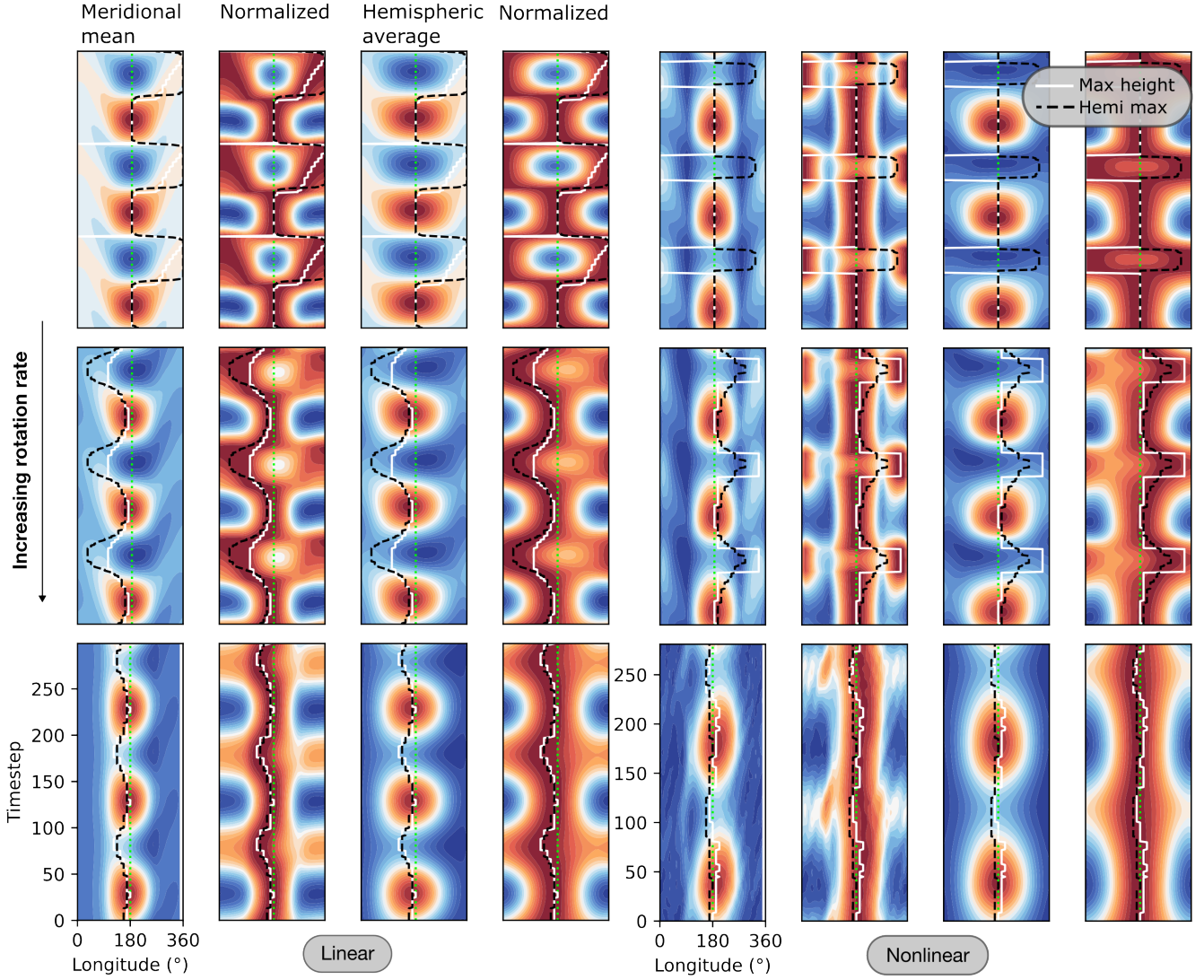
Figure 8. Hovmöller diagrams or timeseries of hotspot location relative to background zonal height profiles for six hot Jupiter planets showing hotspot oscillations switching from westward to eastward with rotation as the system transitions from linear to nonlinear regime. The left column corresponds to \Delta h_{\text{eq}} = 0.001 and the second column to \Delta h_{\text{eq}} = 1 . Each row represents an increasing rotation period (282.9, 14.9 and 1.42 days), and columns show different diagnostic quantities: the meridional mean height, the meridional mean height normalized by the max height at each timestep to expose the instantaneous hotspot location, the hemispheric average height, and similarly normalized hemispheric average. The dotted green line marks the substellar longitude. The colorbars for background height fields are dropped to keep the figure clean focussing on the hotspot locations. White solid lines track the meridional mean-height hotspot, while black dashed lines track the hemispheric-maximum hotspot. The time window shown spans the last 3 forcing periods of the respective simulations.
